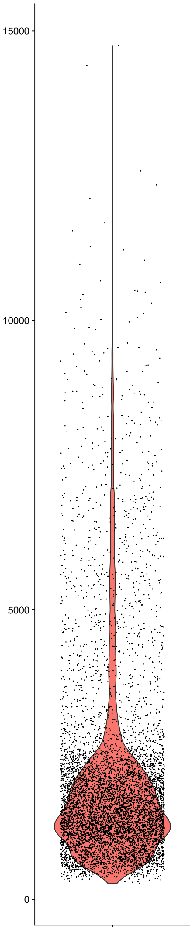
nCount_RNA
