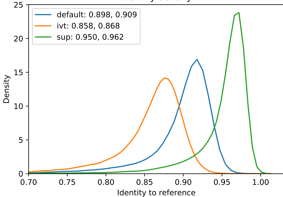
Identity density
