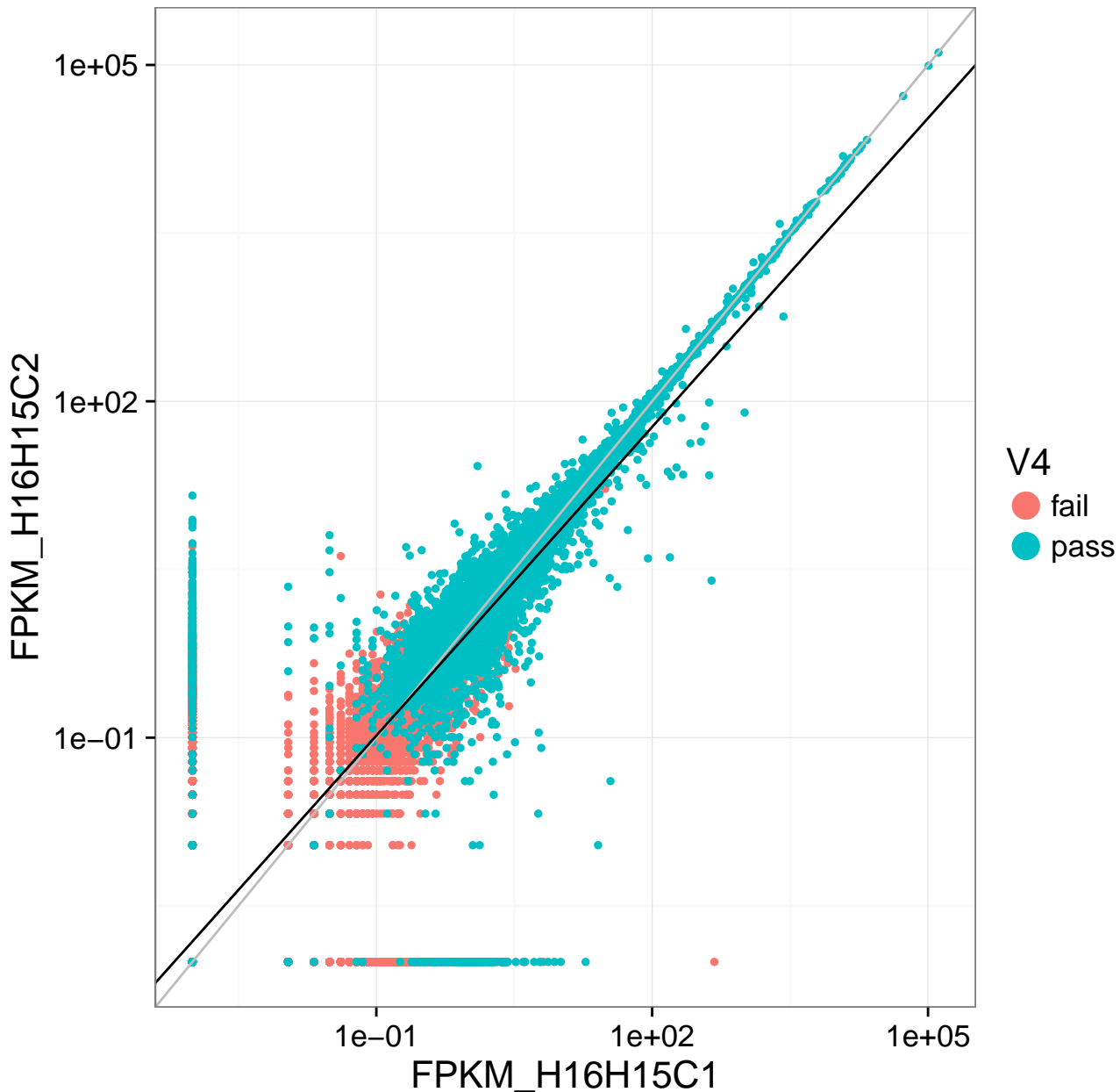
H16H15C1-H16H15C2 (p_r=0.93; s_r=0.93)
