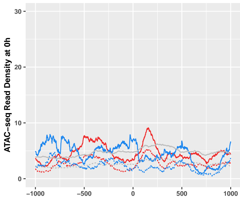
ATAC-seq: Genic-exonic lncRNAs
