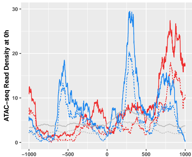
ATAC-seq: Genic-intronic lncRNAs
