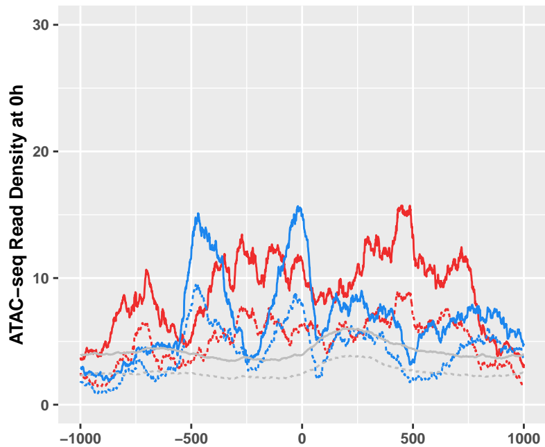
ATAC-seq: Intergenic lncRNAs
