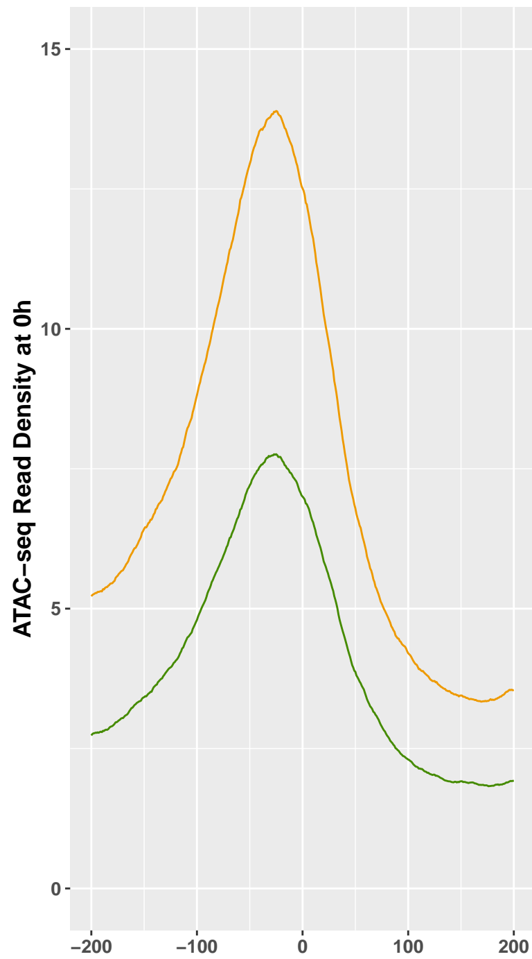
ATAC-seq: mRNA up regulated at 0h
