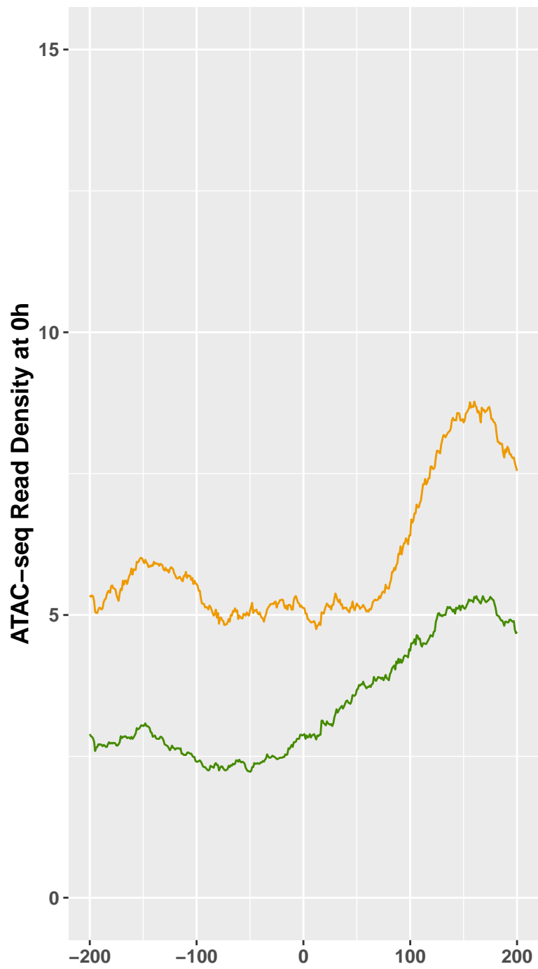
ATAC-seq: lncRNAs up regulated at 0h
