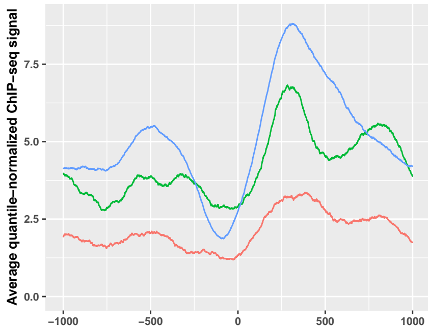
ChIP-seq Control: upregulated genic lncRNAs at 0h (66)
