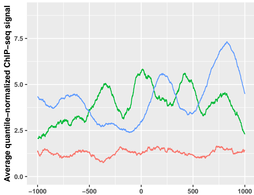
ChIP-seq Control: upregulated intergenic lncRNAs at 0h (18)
