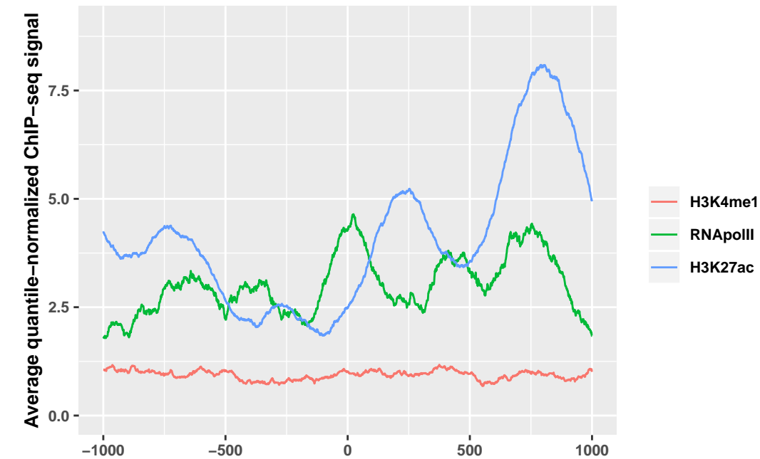
ChIP-seq Regeneration: upregulated intergenic lncRNAs at 0h (18)
