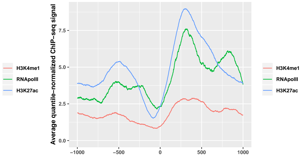
ChIP-seq Regeneration: upregulated genic lncRNAs at 0h (66)
