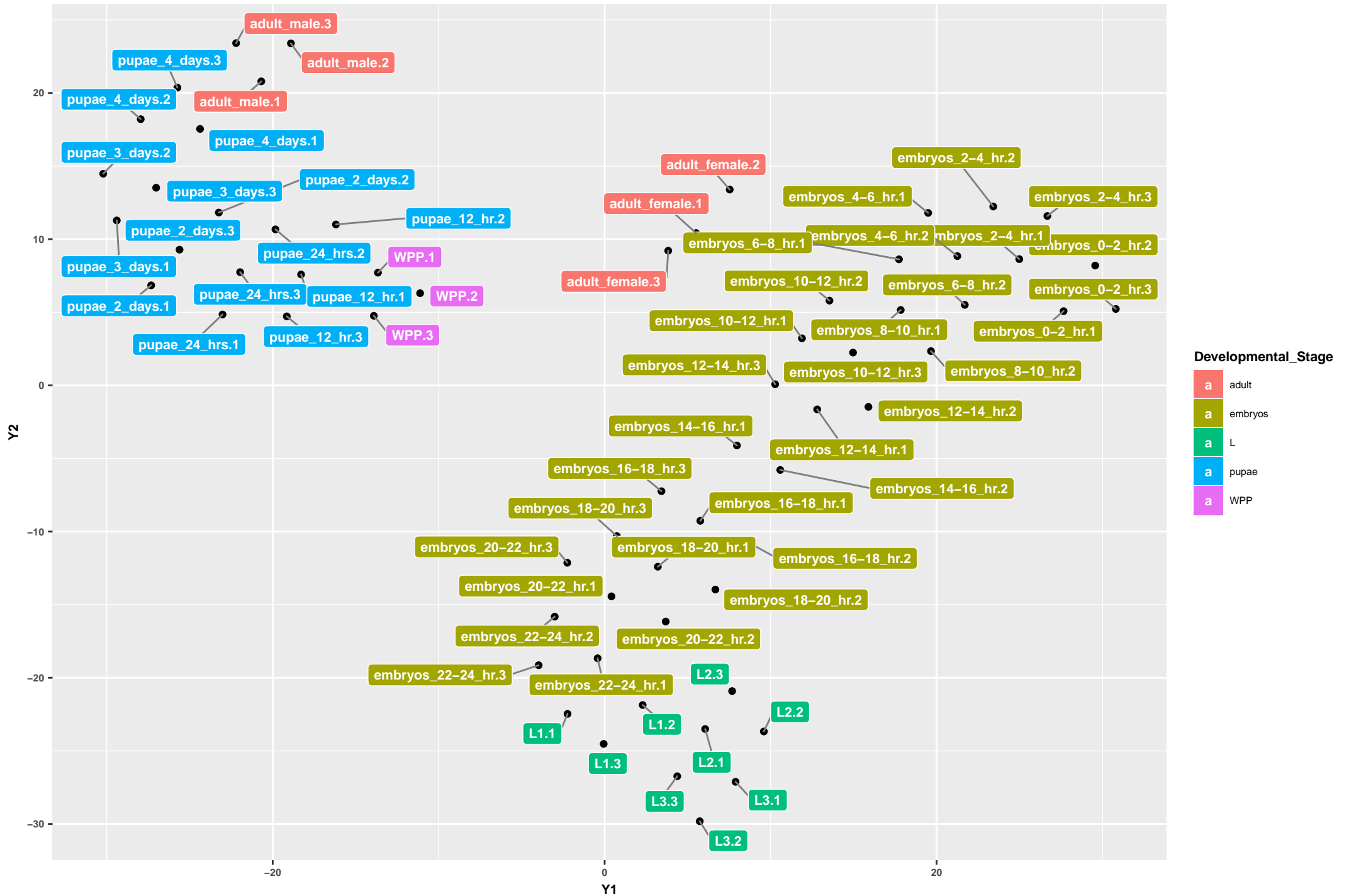
t-SNE: modENCODE development
