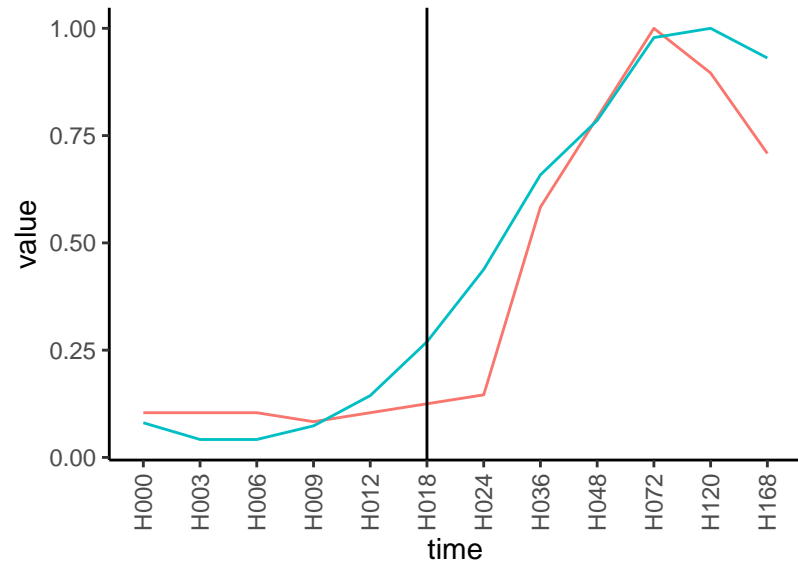
Normalized signals – ENSG00000168329 pre-not-upregulated/post-upregulated
