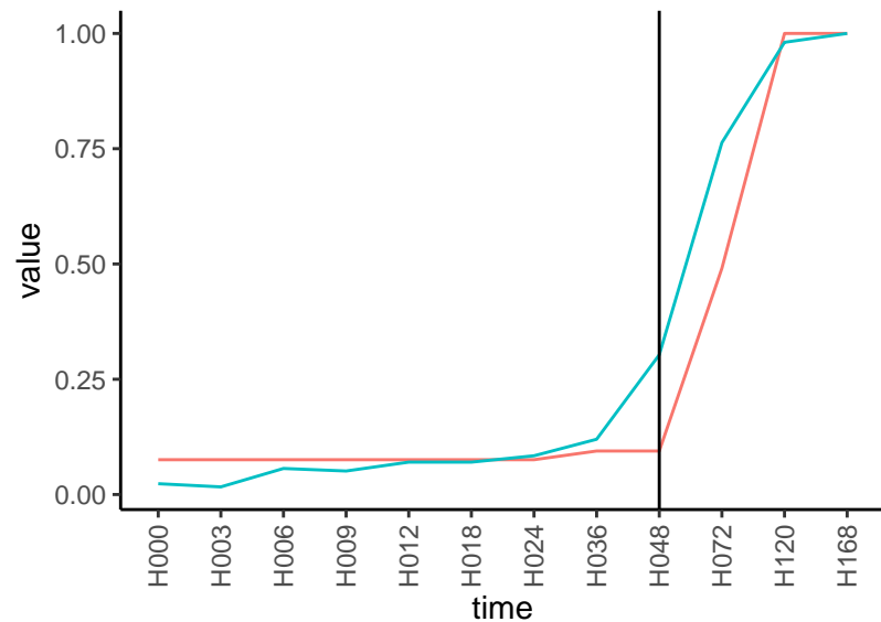
Normalized signals – ENSG00000158714 pre-not-upregulated/post-upregulated
