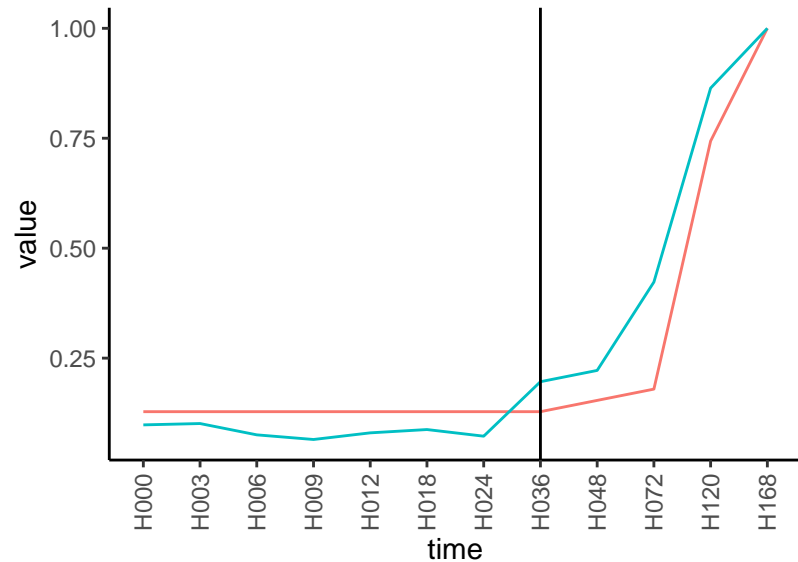
Normalized signals – ENSG00000136250 pre-not-upregulated/post-upregulated
