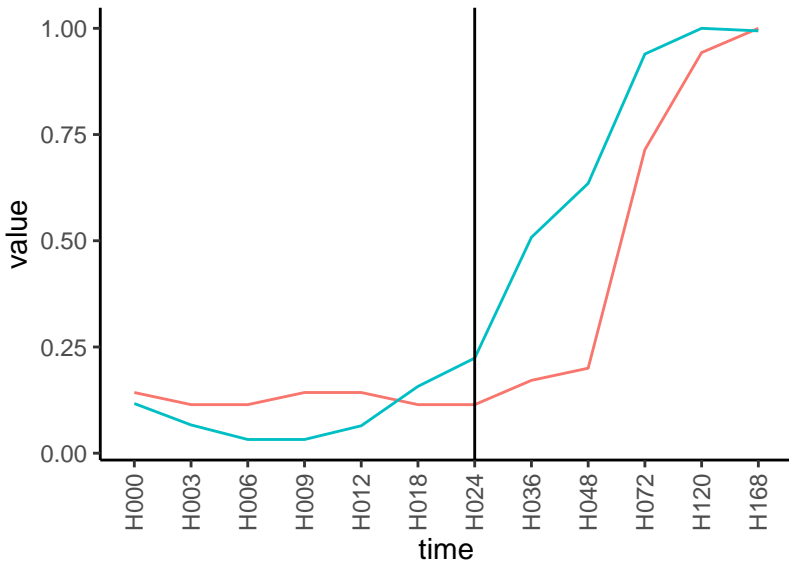
Normalized signals – ENSG00000171777 pre-not-upregulated/post-not-upregulated
