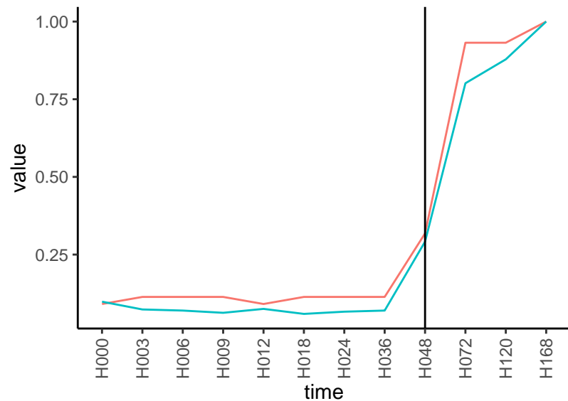
Normalized signals – ENSG00000196730 pre-not-upregulated/post-not-upregulated
