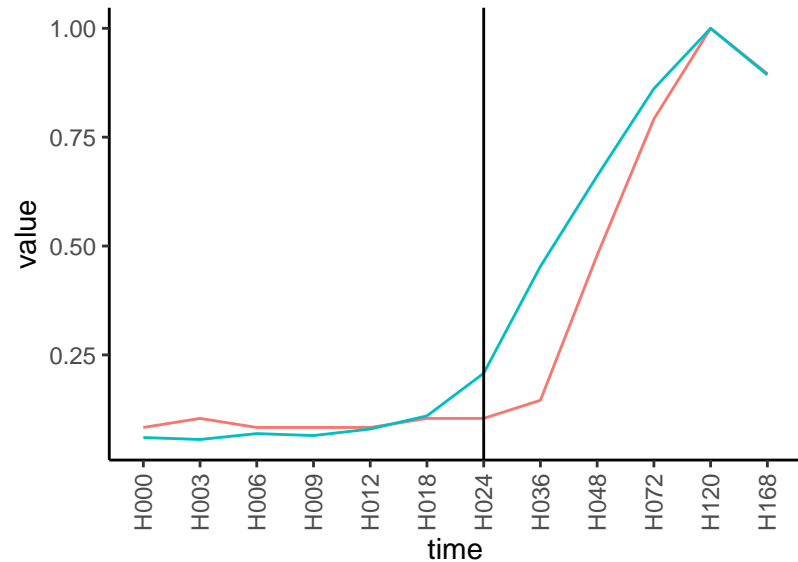
Normalized signals – ENSG00000014257 pre-not-upregulated/post-upregulated
