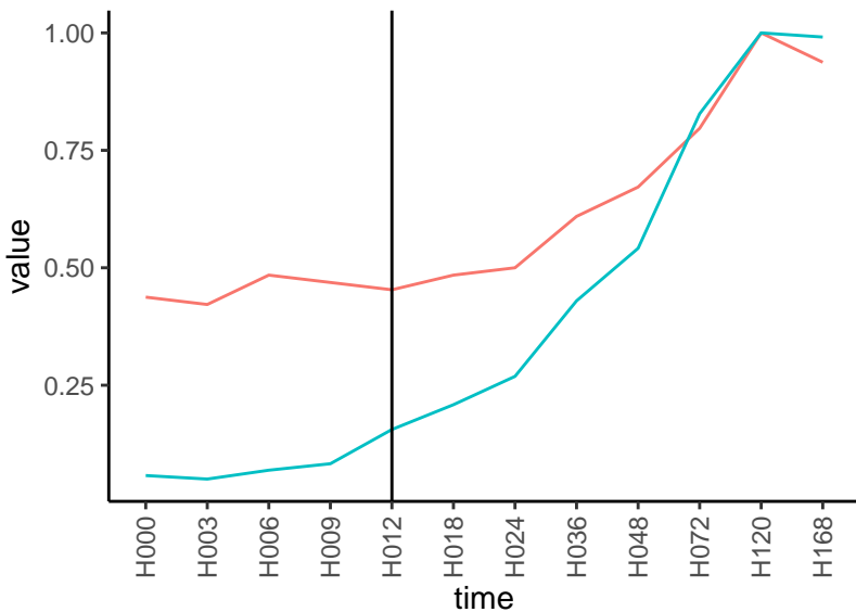
Normalized signals – ENSG00000204577 pre-not-upregulated/post-not-upregulated
