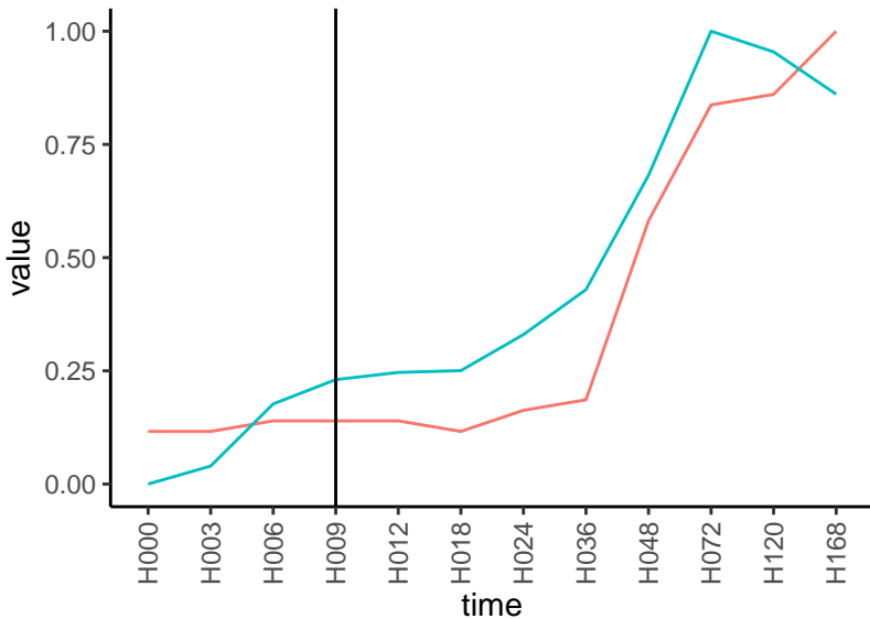
Normalized signals – ENSG00000276600 pre-not-upregulated/post-not-upregulated
