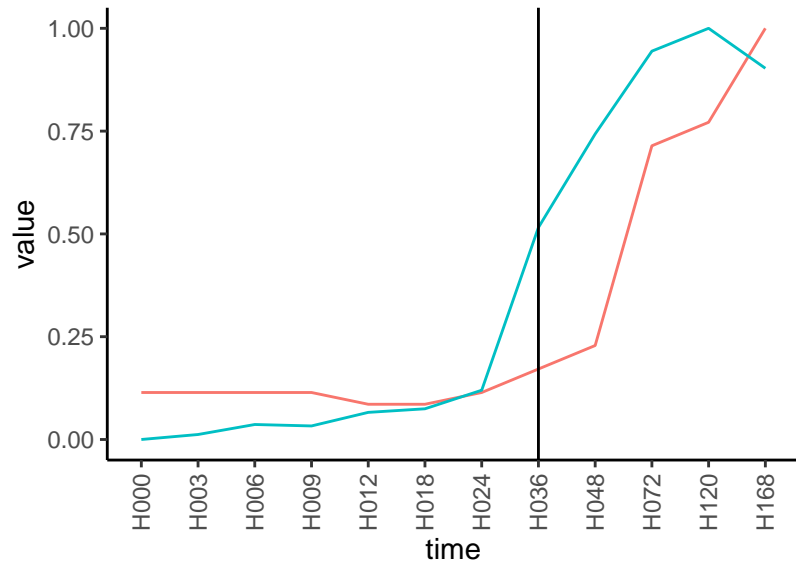
Normalized signals – ENSG00000160791 pre-not-upregulated/post-upregulated
