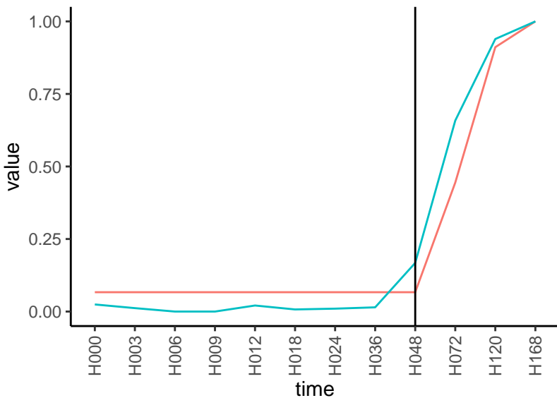
Normalized signals – ENSG00000173369 pre-not-upregulated/post-not-upregulated
