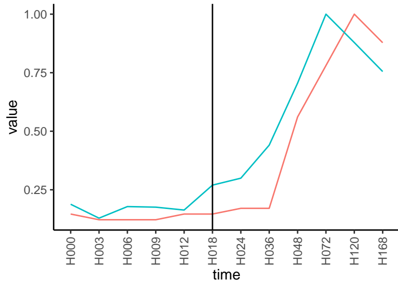
Normalized signals – ENSG00000031081 pre-not-upregulated/post-upregulated
