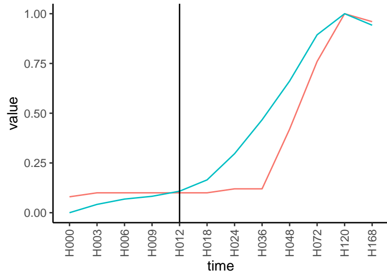
Normalized signals – ENSG00000136689 pre-not-upregulated/post-upregulated
