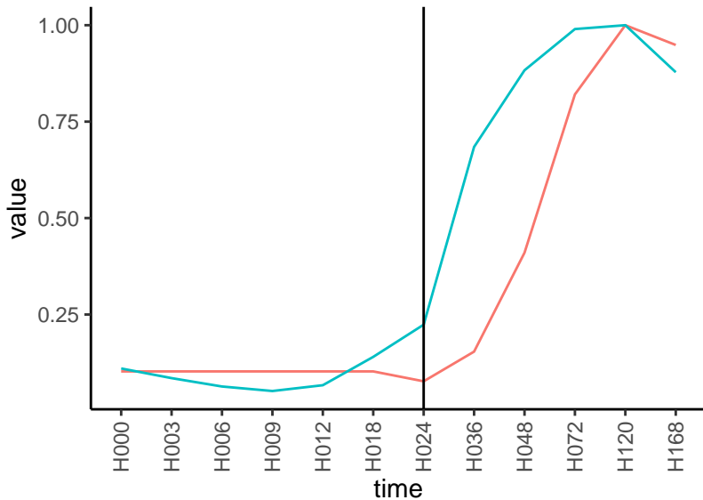
Normalized signals – ENSG00000000938 pre-not-upregulated/post-upregulated
