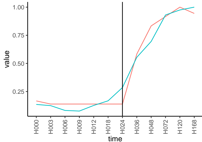
Normalized signals – ENSG00000167851 pre-not-upregulated/post-upregulated
