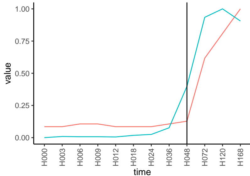
Normalized signals – ENSG00000181634 pre-not-upregulated/post-upregulated
