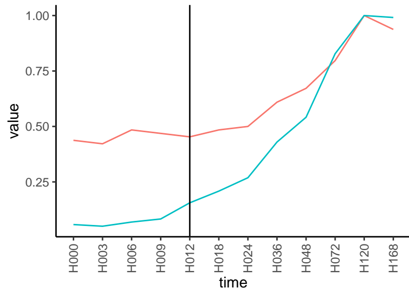
Normalized signals – ENSG00000204577 pre-not-upregulated/post-upregulated
