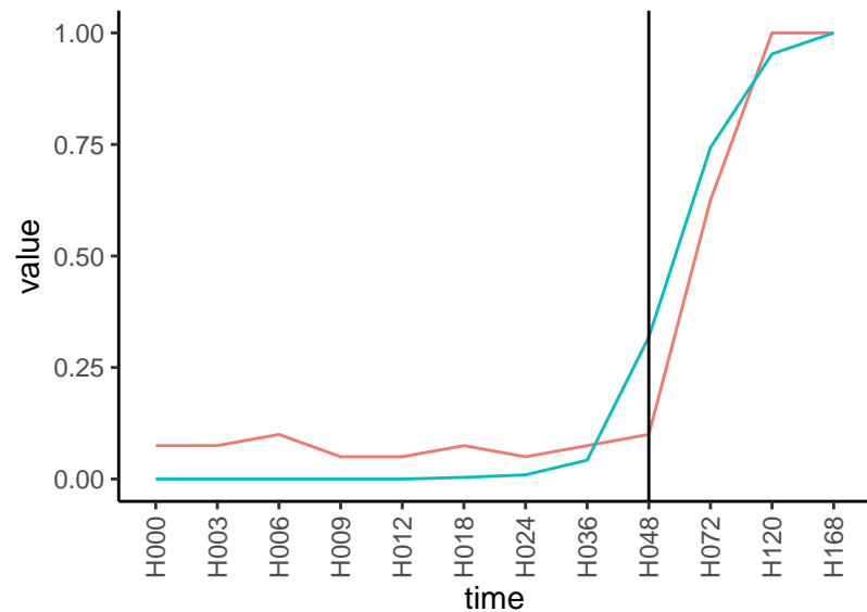
Normalized signals – ENSG00000159189 pre-not-upregulated/post-upregulated
