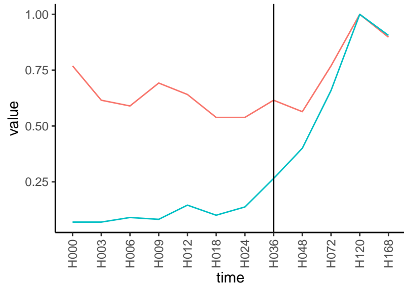
Normalized signals – ENSG00000221869 pre-not-upregulated/post-upregulated
