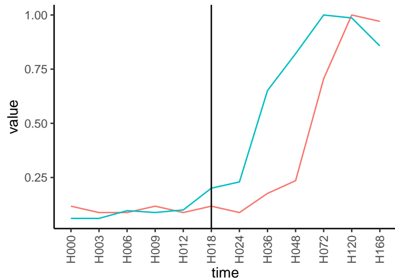
Normalized signals – ENSG00000160883 pre-not-upregulated/post-upregulated
