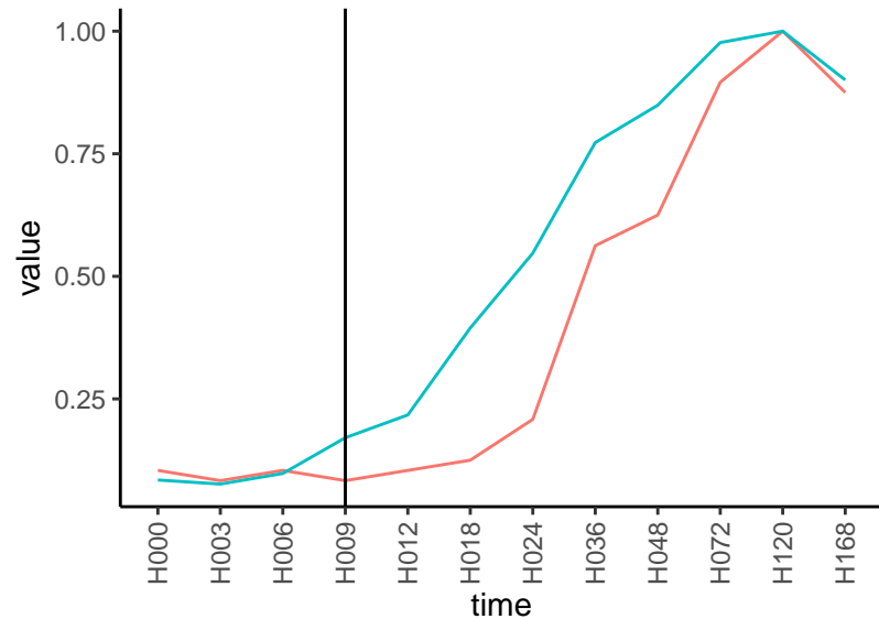
Normalized signals – ENSG00000005844 pre-not-upregulated/post-upregulated
