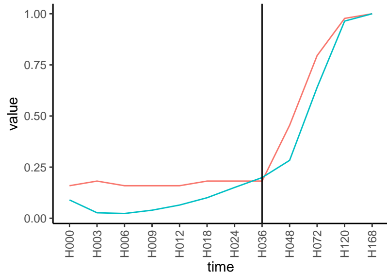
Normalized signals – ENSG00000171115 pre-not-upregulated/post-upregulated
