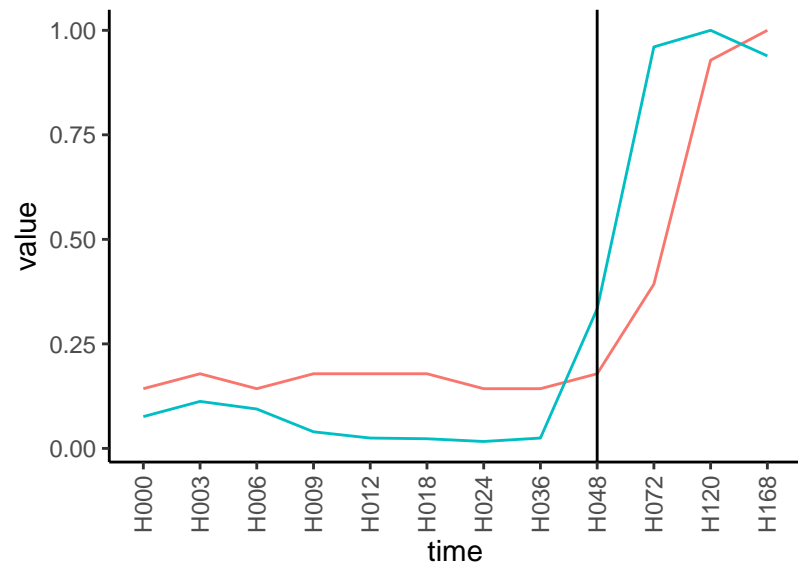
Normalized signals – ENSG00000137801 pre-not-upregulated/post-upregulated
