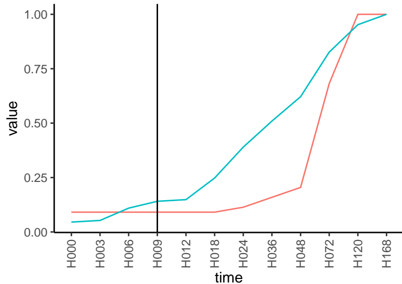
Normalized signals – ENSG00000140678 pre-not-upregulated/post-upregulated
