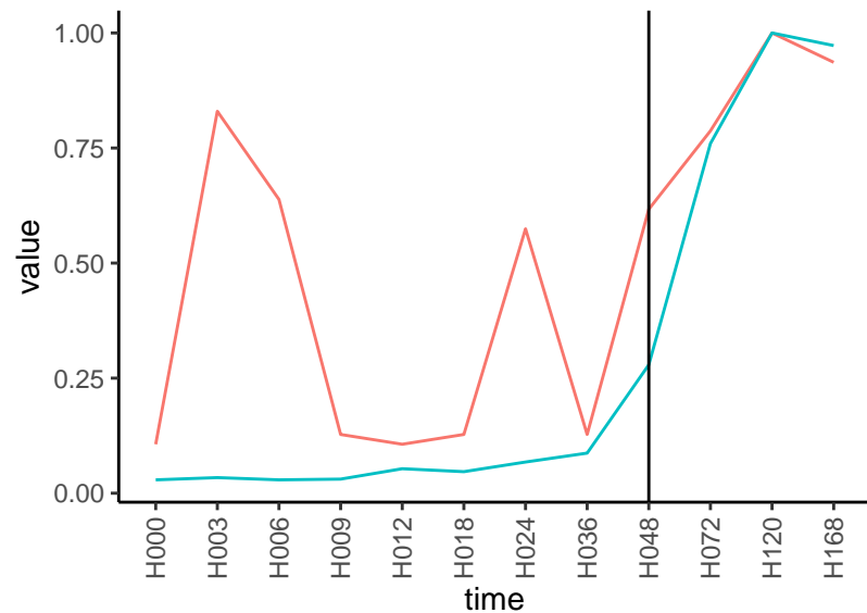
Normalized signals – ENSG00000163694 pre-not-upregulated/post-upregulated
