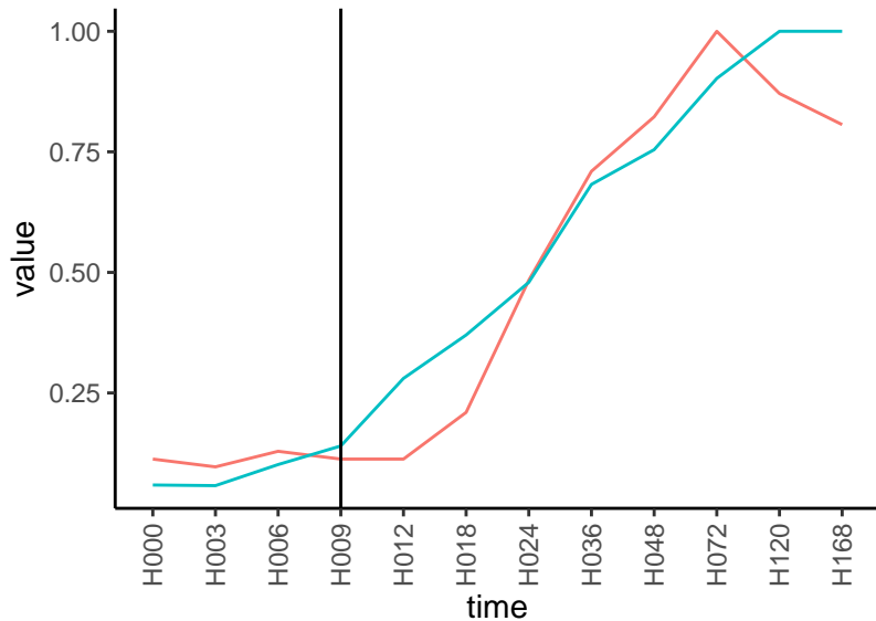
Normalized signals – ENSG00000163823 pre-not-upregulated/post-upregulated
