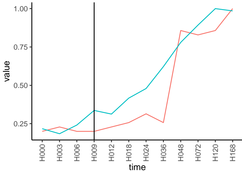
Normalized signals – ENSG00000174130 pre-not-upregulated/post-upregulated
