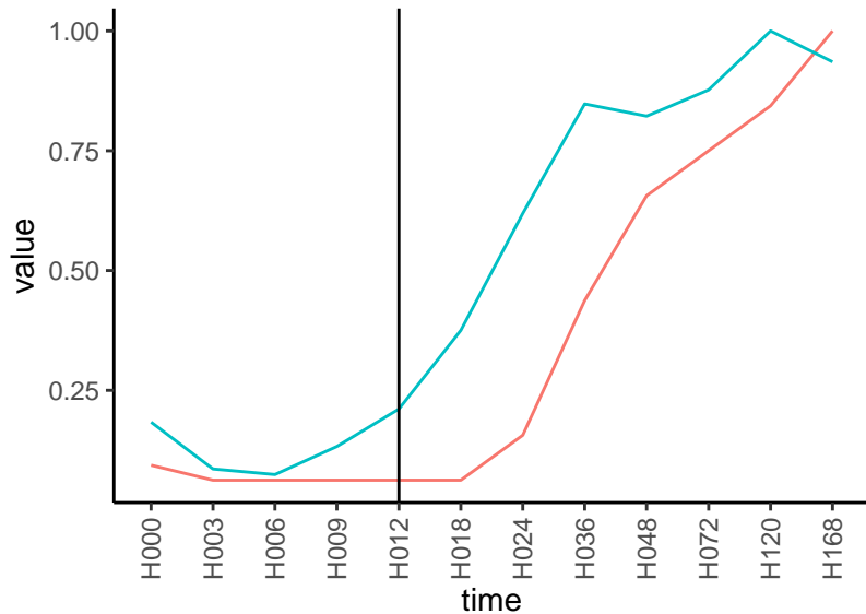
Normalized signals – ENSG00000110665 pre-not-upregulated/post-upregulated
