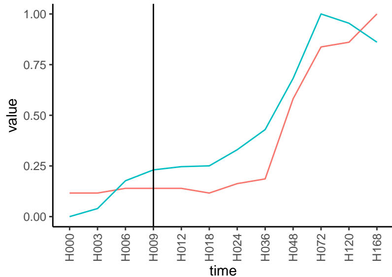
Normalized signals – ENSG00000276600 pre-not-upregulated/post-upregulated
