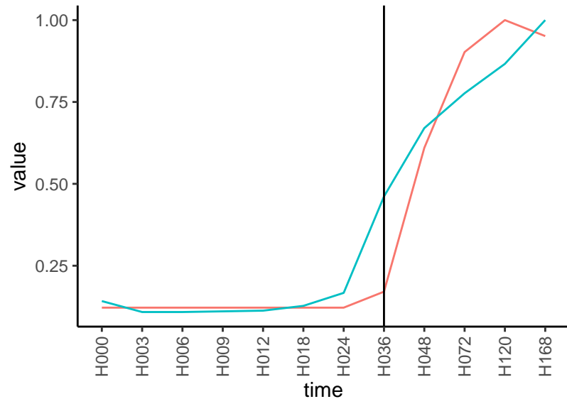
Normalized signals – ENSG00000116574 pre-not-upregulated/post-upregulated
