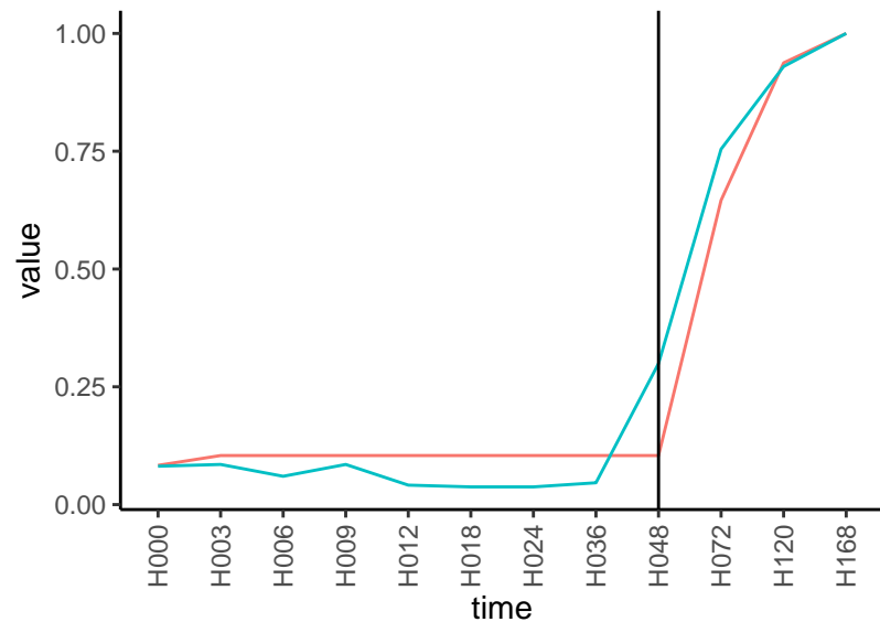
Normalized signals – ENSG00000137491 pre-not-upregulated/post-upregulated
