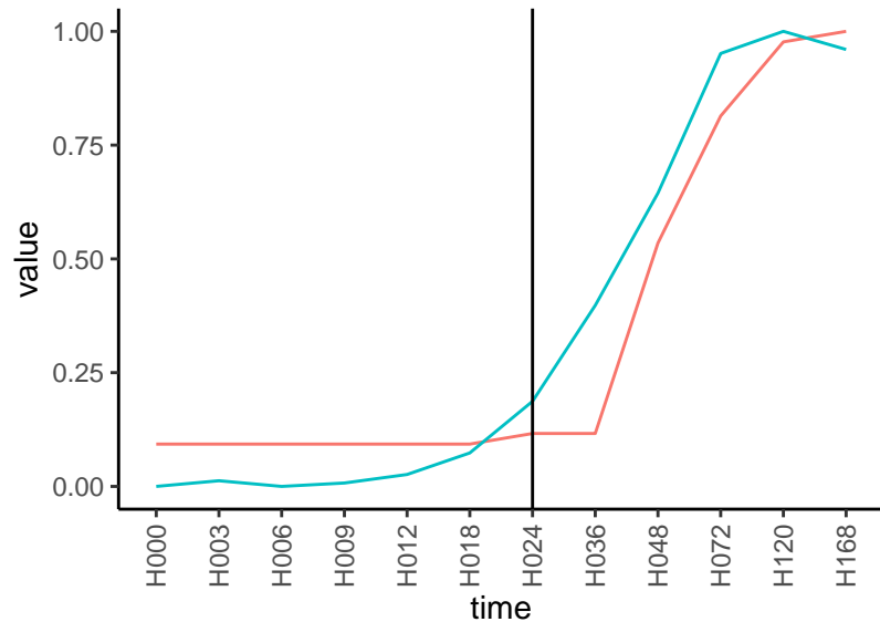
Normalized signals – ENSG00000150540 pre-not-upregulated/post-upregulated
