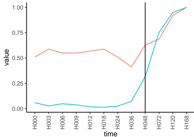
Normalized signals – ENSG00000131981 pre-not-upregulated/post-upregulated
