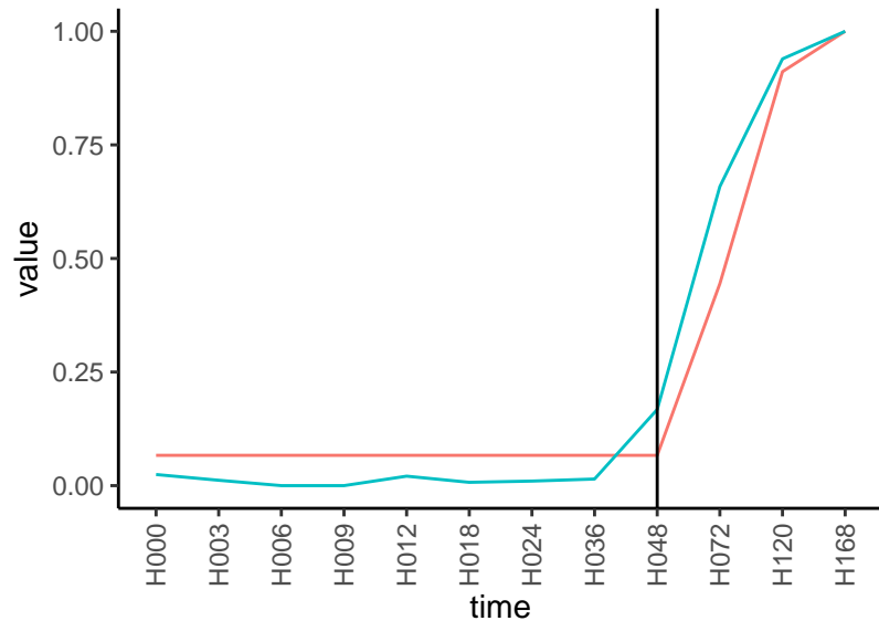
Normalized signals – ENSG00000173369 pre-not-upregulated/post-upregulated
