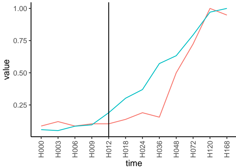
Normalized signals – ENSG00000110077 pre-not-upregulated/post-upregulated
