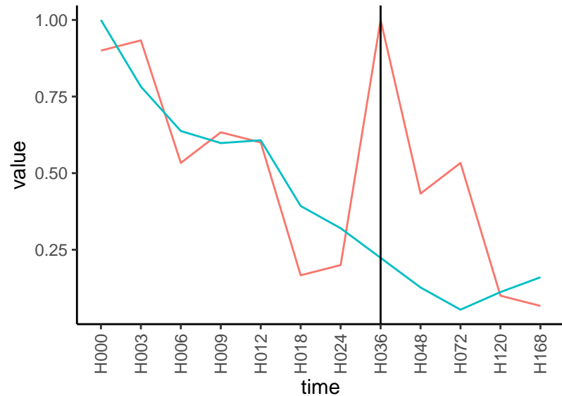
Normalized signals – ENSG00000166159 pre-not-downregulated/post-downregulated
