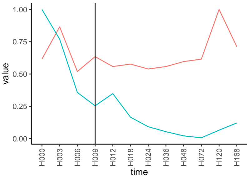
Normalized signals – ENSG00000198821 pre-not-downregulated/post-not-downregula
