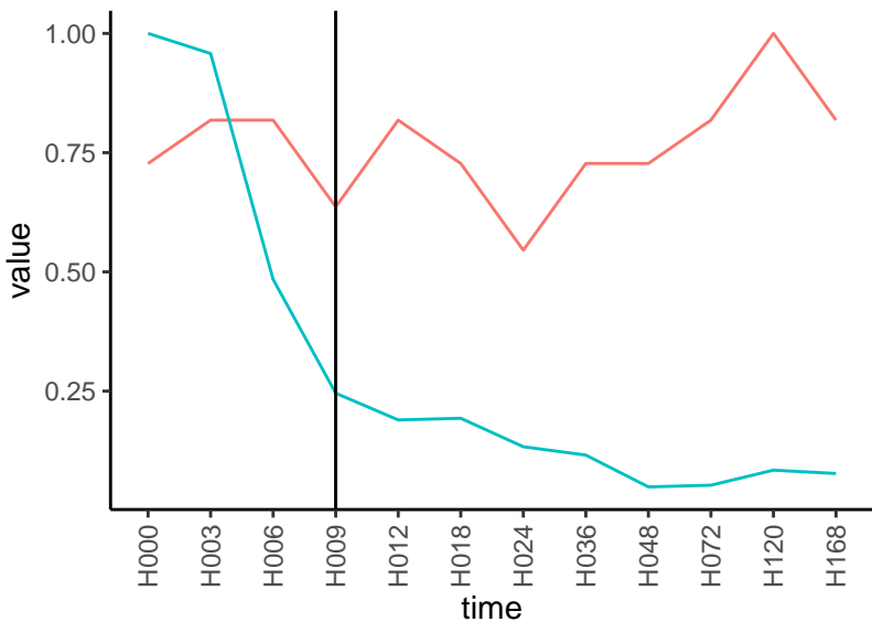
Normalized signals – ENSG00000132185 pre-not-downregulated/post-not-downregula
