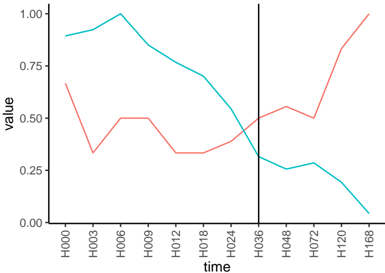
Normalized signals – ENSG00000154545 pre-not-downregulated/post-not-downregula
