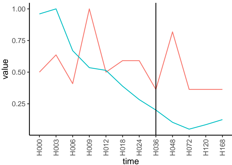
Normalized signals – ENSG00000185737 pre-not-downregulated/post-not-downregula
