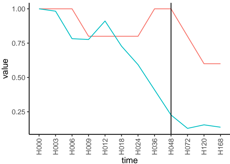
Normalized signals – ENSG00000114631 pre-not-downregulated/post-not-downregula
