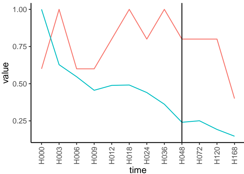
Normalized signals – ENSG00000185271 pre-not-downregulated/post-downregulated
