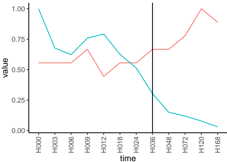
Normalized signals – ENSG00000145911 pre-not-downregulated/post-not-downregula
