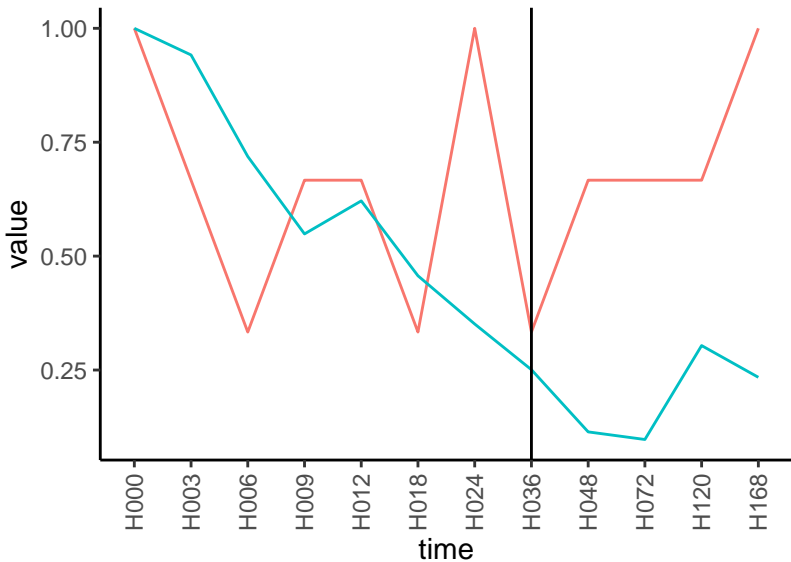
Normalized signals – ENSG00000117122 pre-not-downregulated/post-not-downregula
