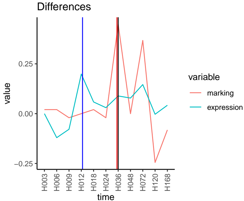
Normalized signals – ENSG00000101439 pre-not-upregulated/post-not-upregulated
