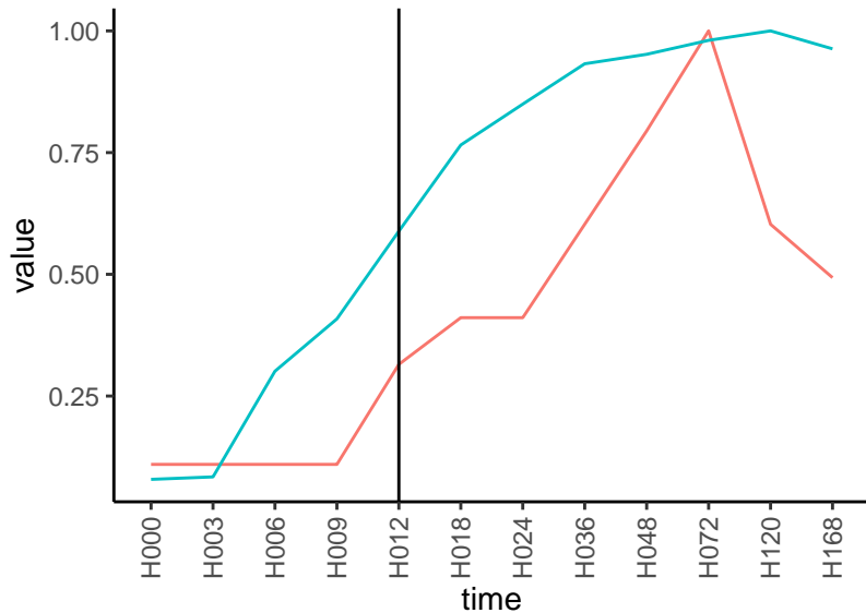
Normalized signals – ENSG00000010327 pre-not-upregulated/post-upregulated
