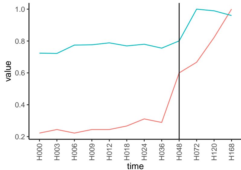
Normalized signals – ENSG00000176871 pre-not-upregulated/post-not-upregulated
