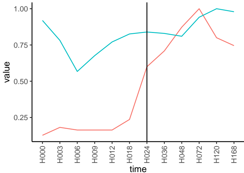
Normalized signals – ENSG00000111679 pre-not-upregulated/post-not-upregulated
