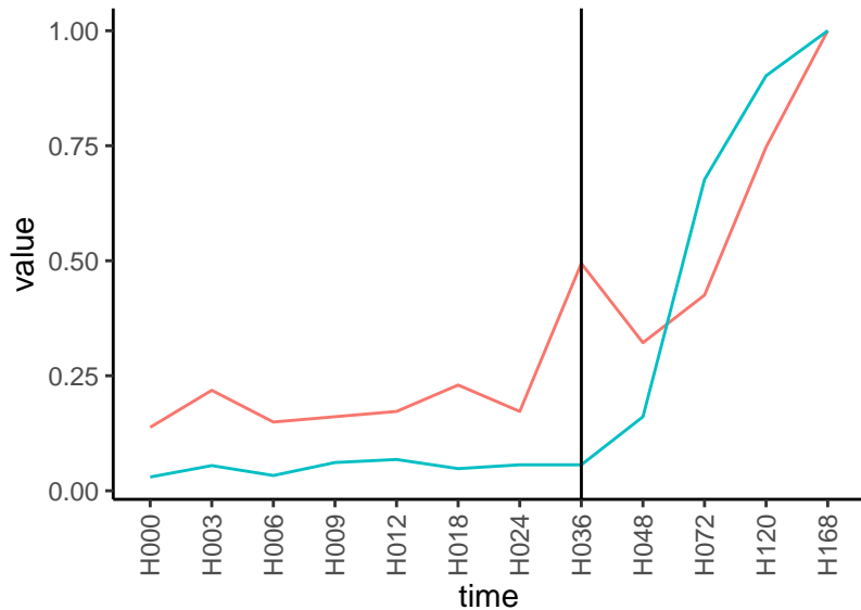
Normalized signals – ENSG00000171227 pre-not-upregulated/post-upregulated
