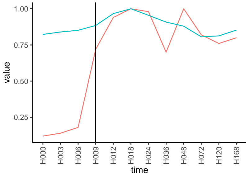
Normalized signals – ENSG00000128973 pre-not-upregulated/post-not-upregulated
