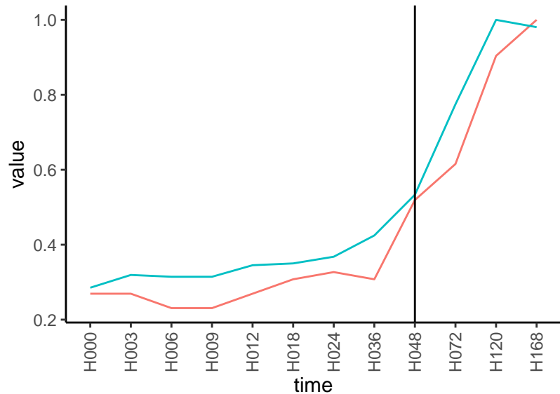
Normalized signals – ENSG00000136867 pre-not-upregulated/post-not-upregulated
