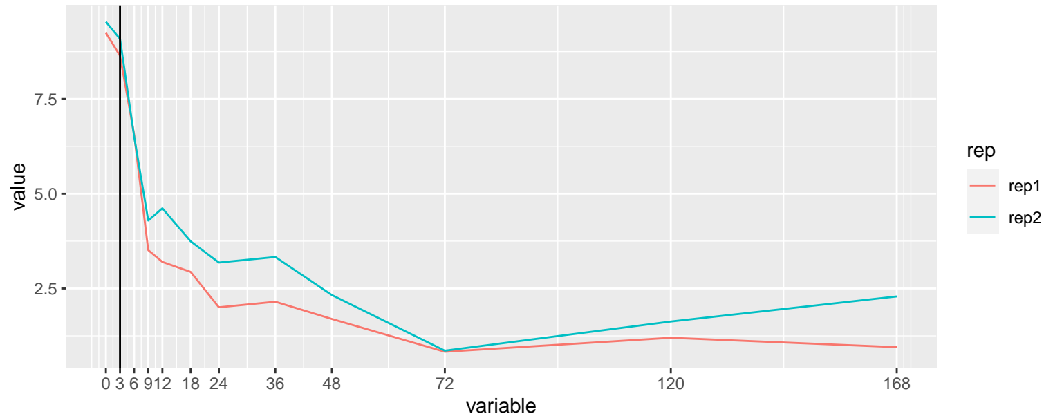
Regression: ENSG00000128322 – H3K4me1
