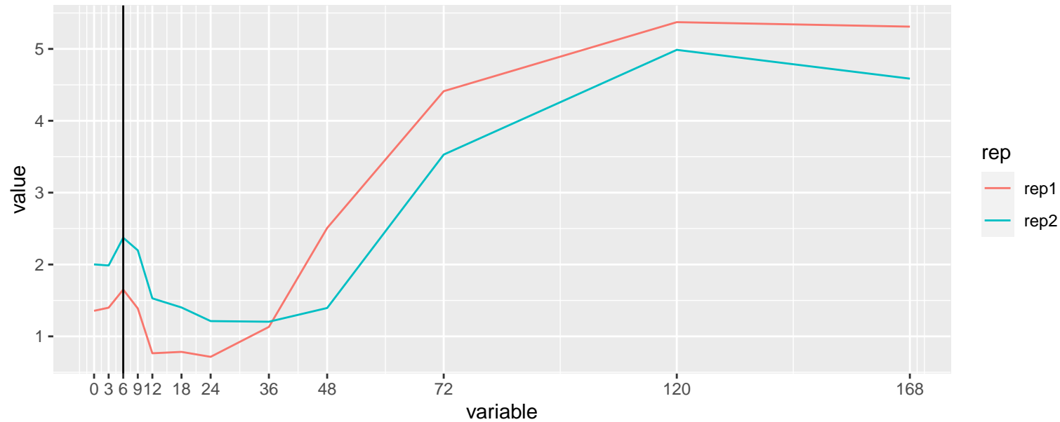
Regression: ENSG00000158186 – H3K4me1
