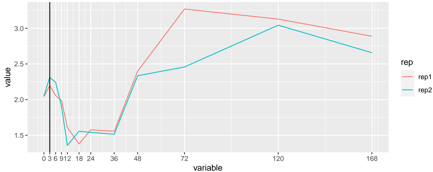
Regression: ENSG00000165338 – H3K4me1
