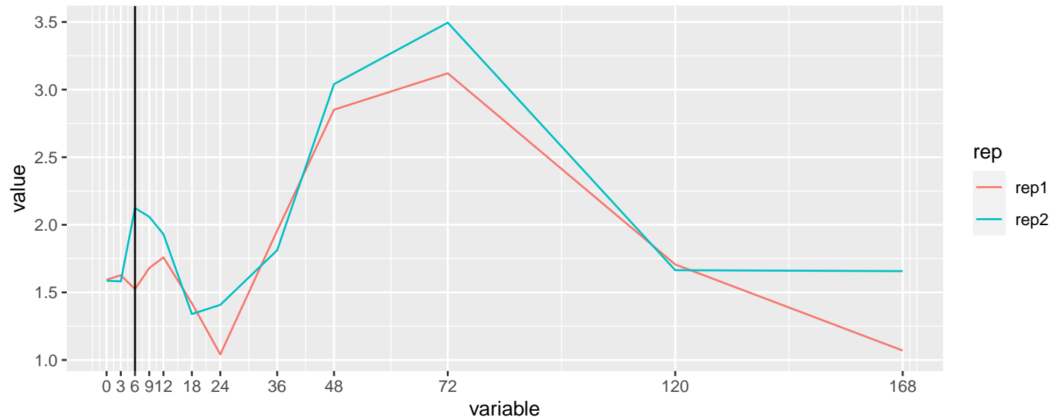
Inconsistent: ENSG00000114948 – H3K4me1
