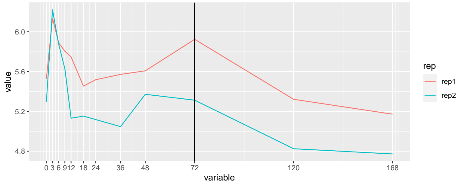
Regression: ENSG00000133731 – H3K4me1
