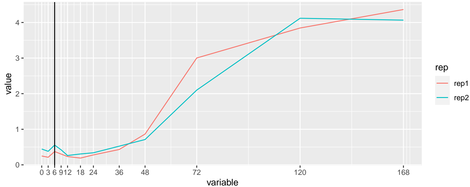
Regression: ENSG00000090376 – H3K4me1
